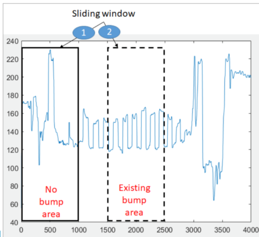
Fig.7: Sliding window
